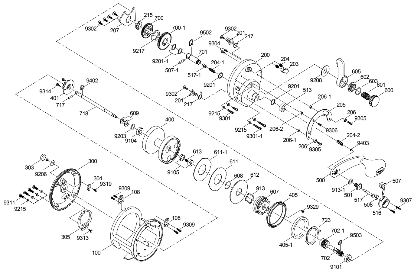
TG - 15 - II (2 of 2) Spare Parts
